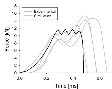
Figure 12: Single Lap-Shear tests, v_{test} = 5000 mm/s
