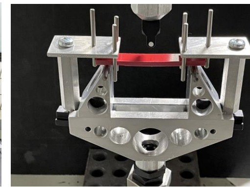
Hipshield bending tests
