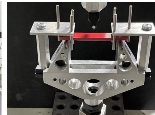
Hipshield bending tests
